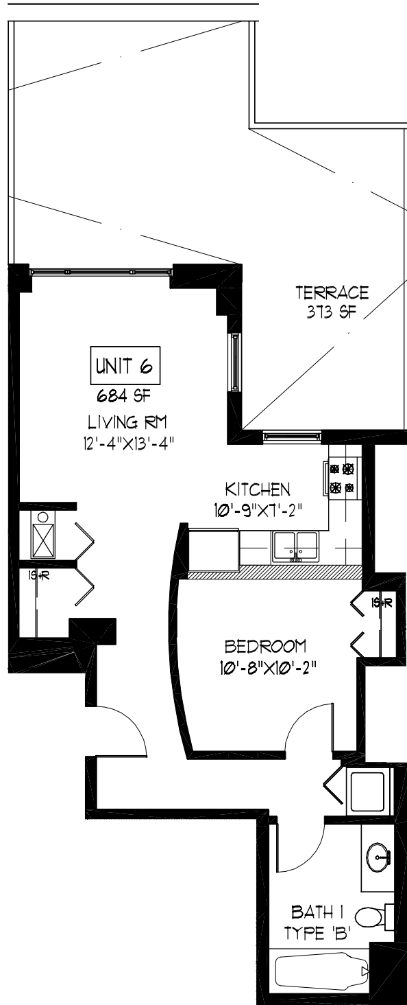
1 UNIT 406 PLAN 1/8" = 1'-0"
